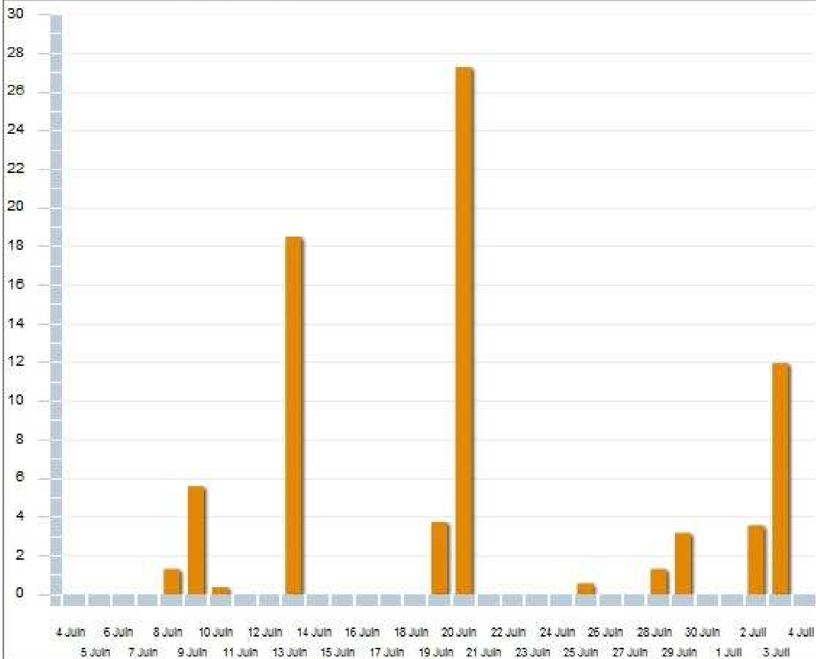
30-day rainfall - June 2013
